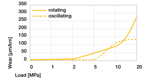
Diagram 07: Wear for oscillating and rotating applications with shaft material C153 hardened and ground steel, as a function of the load
