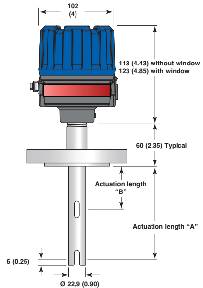
962 - Flanged connection
