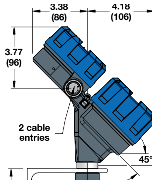
Eclipse® Housing (45° View)
