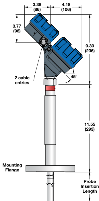
Model 7yS with flanged connection
