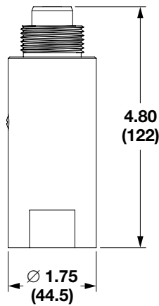
Model 705 Probe Adapter
