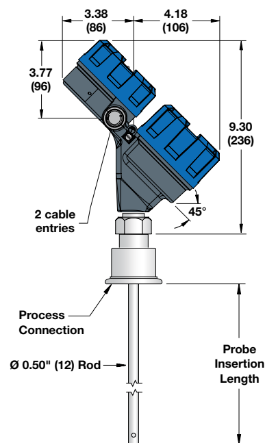
Model 7yH with hygienic connection
