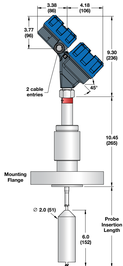
Model 7y6 with flanged connection
