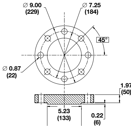
Fisher 249B/259B (600 lb.), carbon steel
