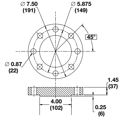
Masoneilan (600 lb.), carbon steel
