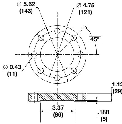
Fisher 249C (600 lb.), 316 stainless steel
