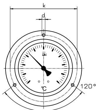
Hole diagram for front flange
