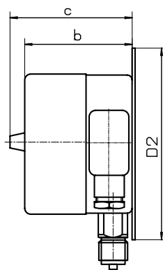
rear mounting flange
