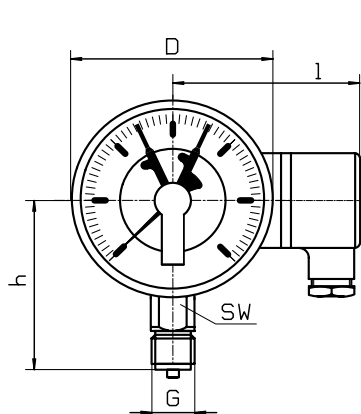
Connection bottom
