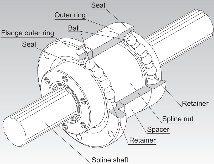
Fig.1 Structure of Rotary Ball Spline Model LTR
