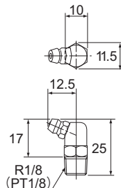
B-PT1/8 type
