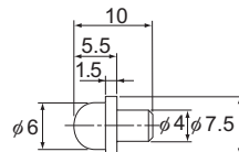
PB1021B type
