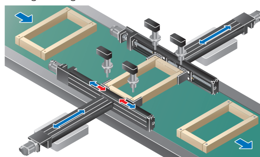
Screw tightening machine
