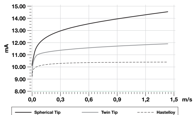
Typical water flow
