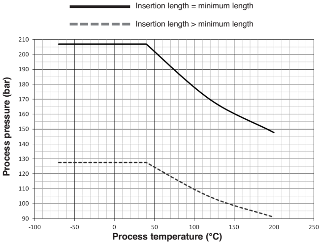
TMC/TMD sensors with material code A or D
