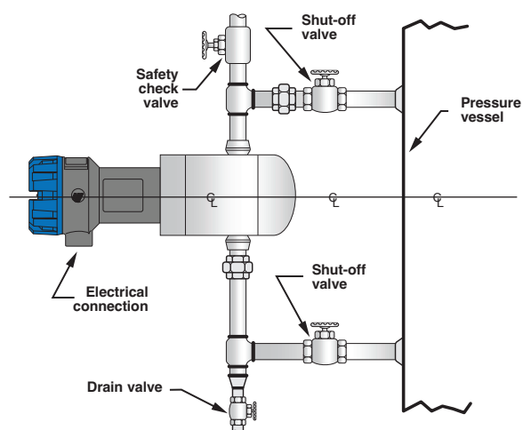
Typical piping arrangement
