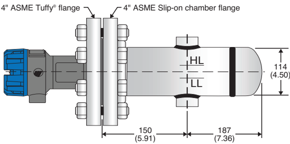
Flanged cage 035
