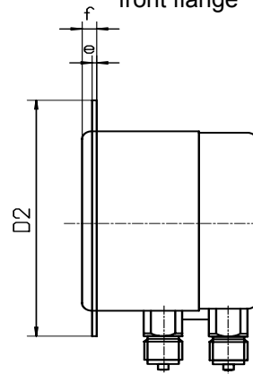
front flange
