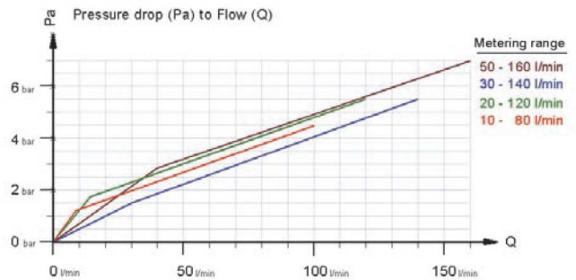
Metering spaces of the flow switch HR2VK1
