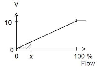
Voltage output
