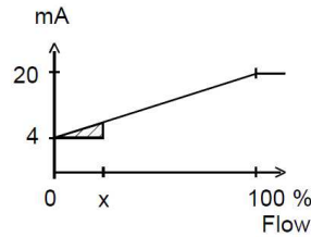
Current output
