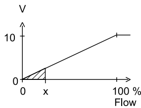
Voltage output
