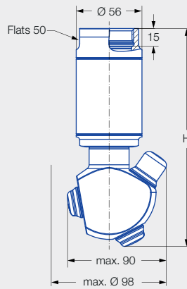
Female thread
