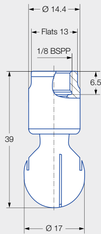
Female thread
