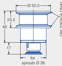
Male thread
