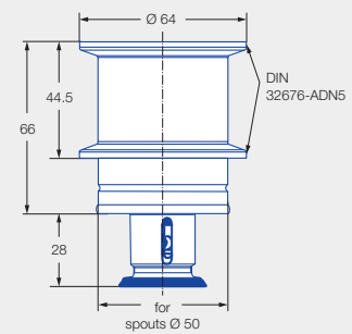
Tri-Clamp connection 2
