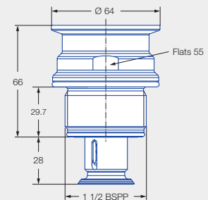
Male thread
