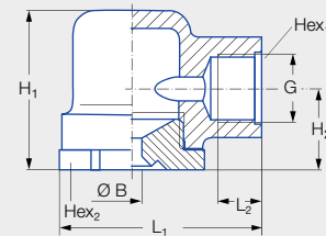
Type 302.52x-302.96x
